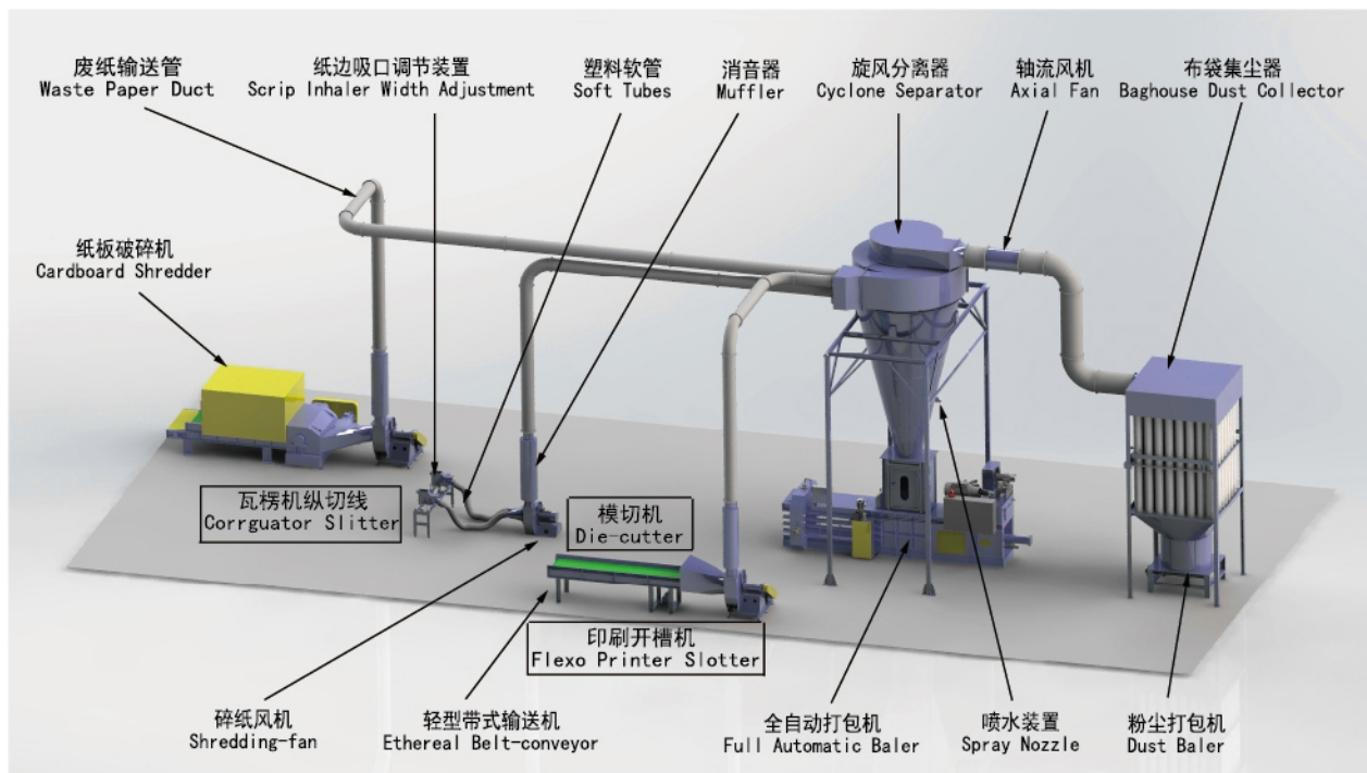
瓦楞纸箱行业整厂废纸处理系统示意图 The Diagram of Packaging Waste Management Systems
