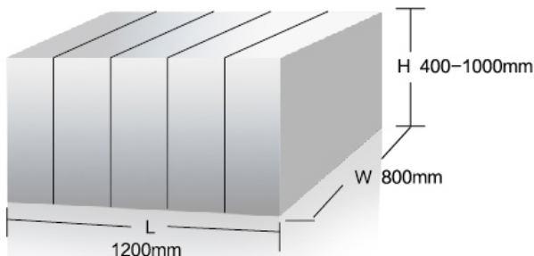
Bale Size ( Model XTY-1200LA12080 )
