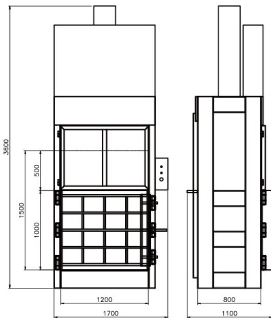
Diagram ( Model XTY-1200LA12080 )
