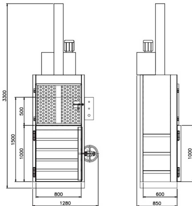
Diagram(Model XTY-300KL8060)
